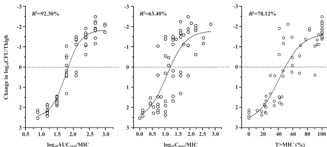
Figure 2. The relationships of the antofloxacin hydrochloride AUC_{24\text{ h}}/\text{MIC} , the percentage of the dosing interval that serum drug concentration remained above the MIC [ T > \text{MIC} (%)], and the C_{\text{max}}/\text{MIC} for S aureus ATCC 29213 with the \log_{10}\text{CFU}/\text{thigh} change after 24 h of therapy. Each point represents the mean value of two thighs from one mouse. R^2 , coefficient of determination. The dotted line indicates the number of bacteria at the start of therapy.
